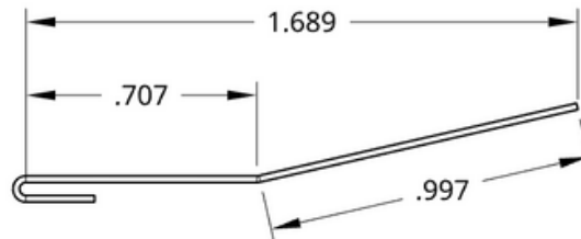
.024" Galvanized Steel Clip
