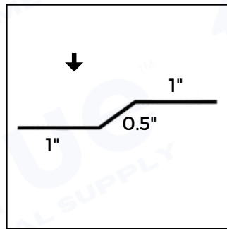
Offset Cleat
