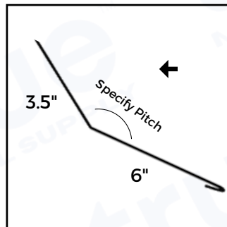
Transition/Pitch Break
