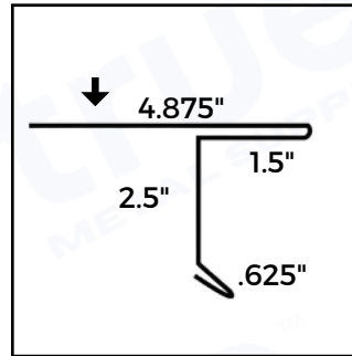
Extended Eave
