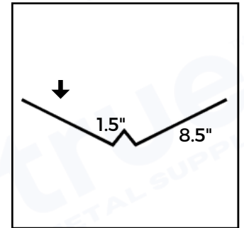
Valley Flashing
