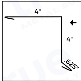
Corner / Rake Trim
