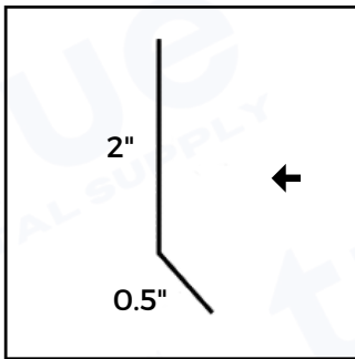
Cleat
