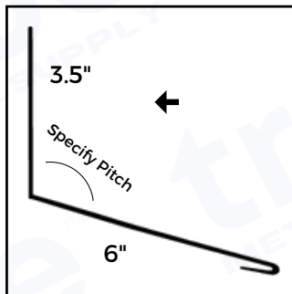
Endwall / Headwall
