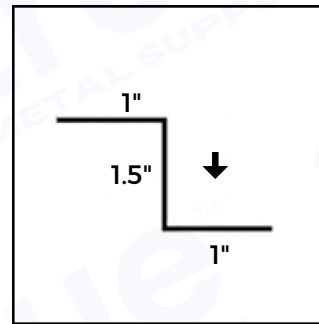
Z-Channel
