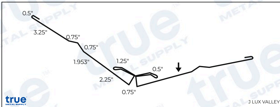
J-Valley
