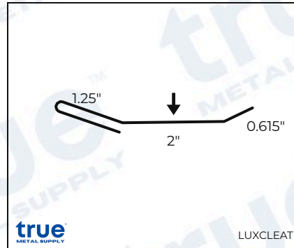
Cleat
