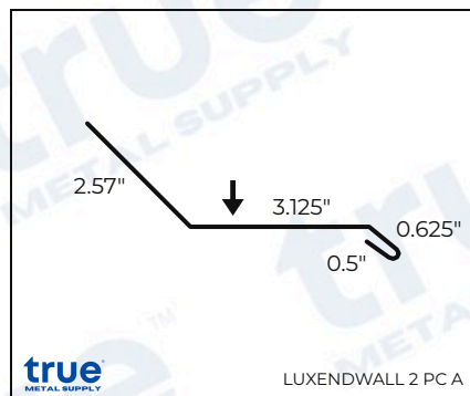
Endwall Flashing (Pc A)
