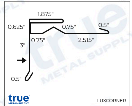
Corner Trim
