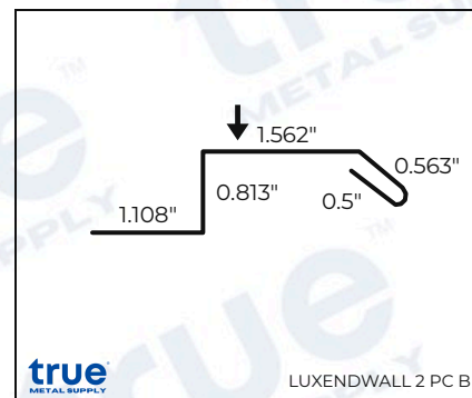
Endwall Flashing (Pc B)
