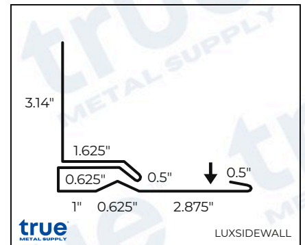
Sidewall Flashing
